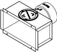
Frontansicht | Front view
