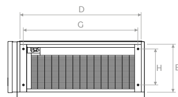
Frontansicht | Front view
