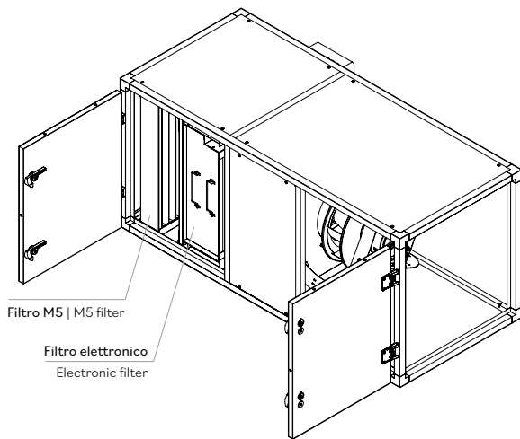
Vista posteriore | Rear view
