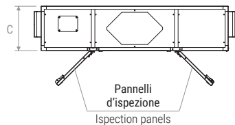
Vista superiore | Upper view
