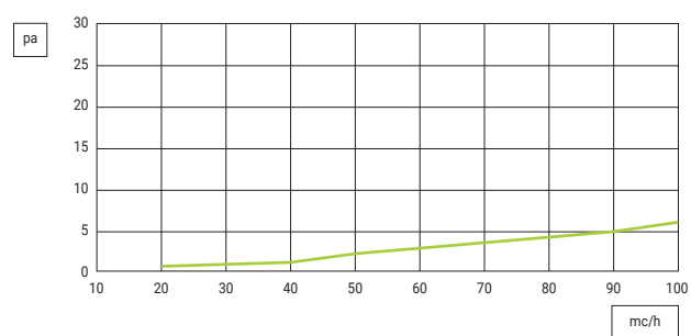
ATTACCHI POSTERIORI | REAR SPIGOTS
