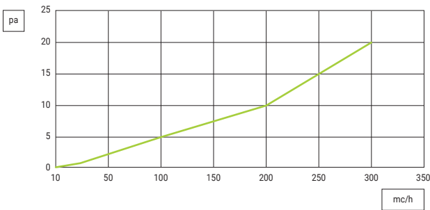
PLUGPVMCSH10 ATTACCHI LATERALI | SIDE SPIGOTS
